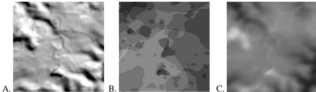
Figure 3. Examples of “mole run” artifacts in an ASTER GDEM shaded-relief image (A) that are clearly related to the stack number boundaries (B). Mole runs, particularly, are less apparent in the normal intensity ASTER GDEM images (C).
